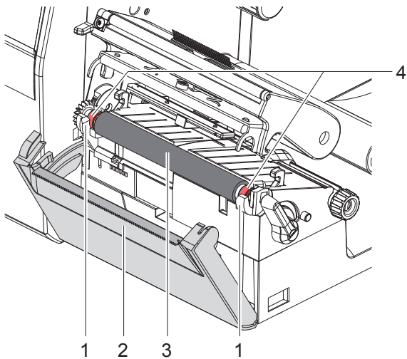
Figure 15 Print roller
