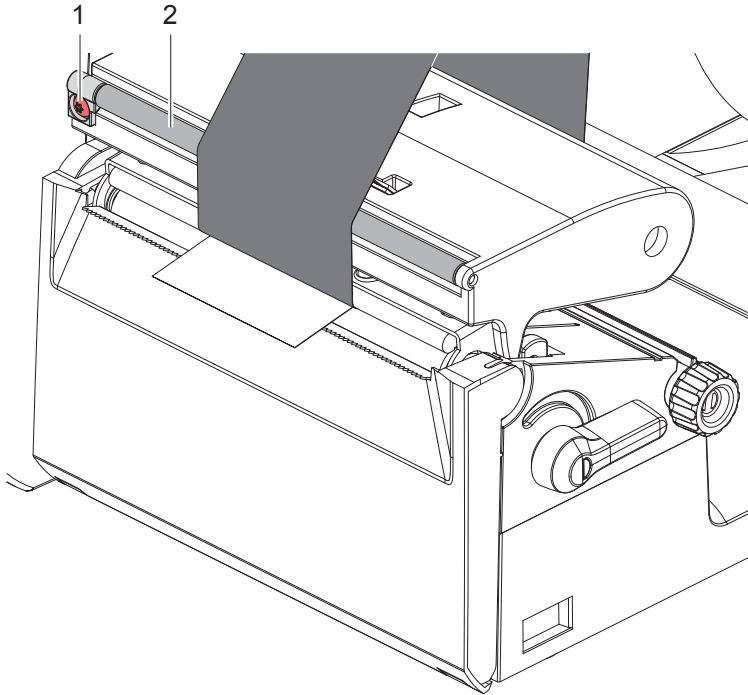
Figure 14 Setting the feed path of the transfer ribbon
