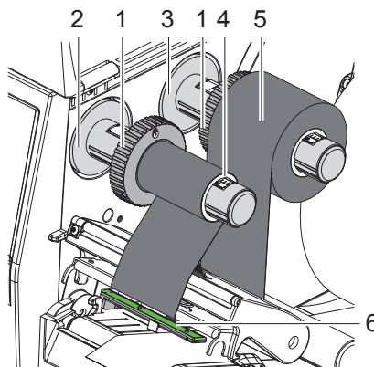
Figure 12 Loading Transfer Ribbon
