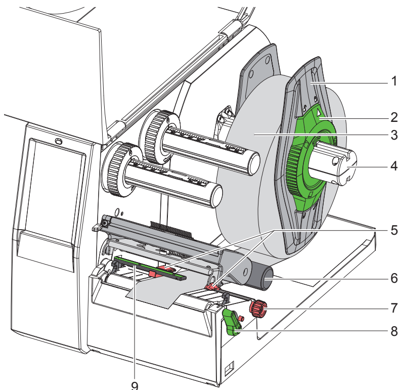
Figure 9 Loading media from roll
