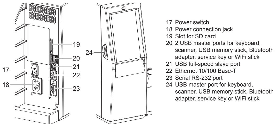
Figure 3 Connections
