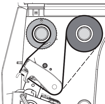
Figure 13 Transfer Ribbon Feed Path
