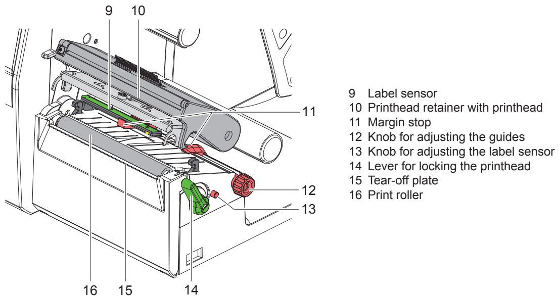
Figure 2 Print unit
