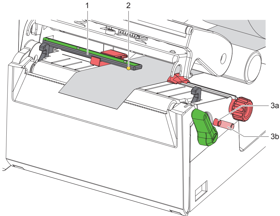
Figure 10 Adjusting the label sensor
